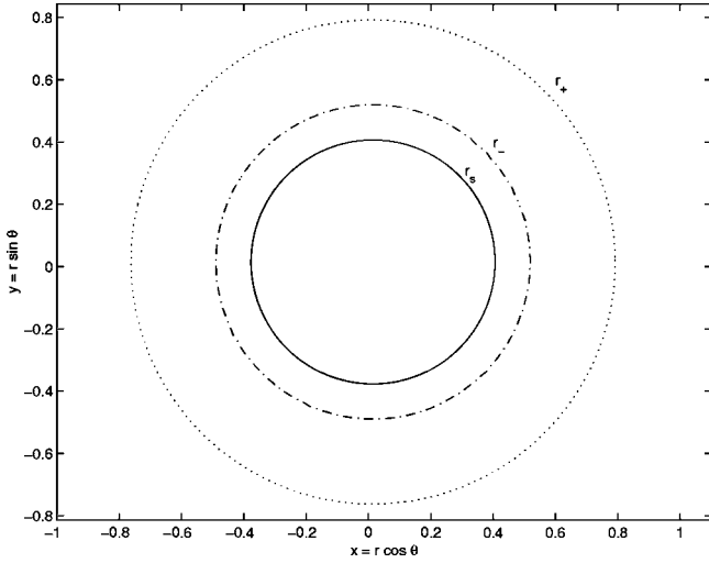
FIG. 1. The singularity and horizons of the toroidal 3D spacetime in the coordinates of metric (37). The parameters are such that the event horizon at r_+ (dotted line) and Cauchy horizon at r_- (dash-dotted line) are present. Spacetime ends at the singularity r_s (full line).
